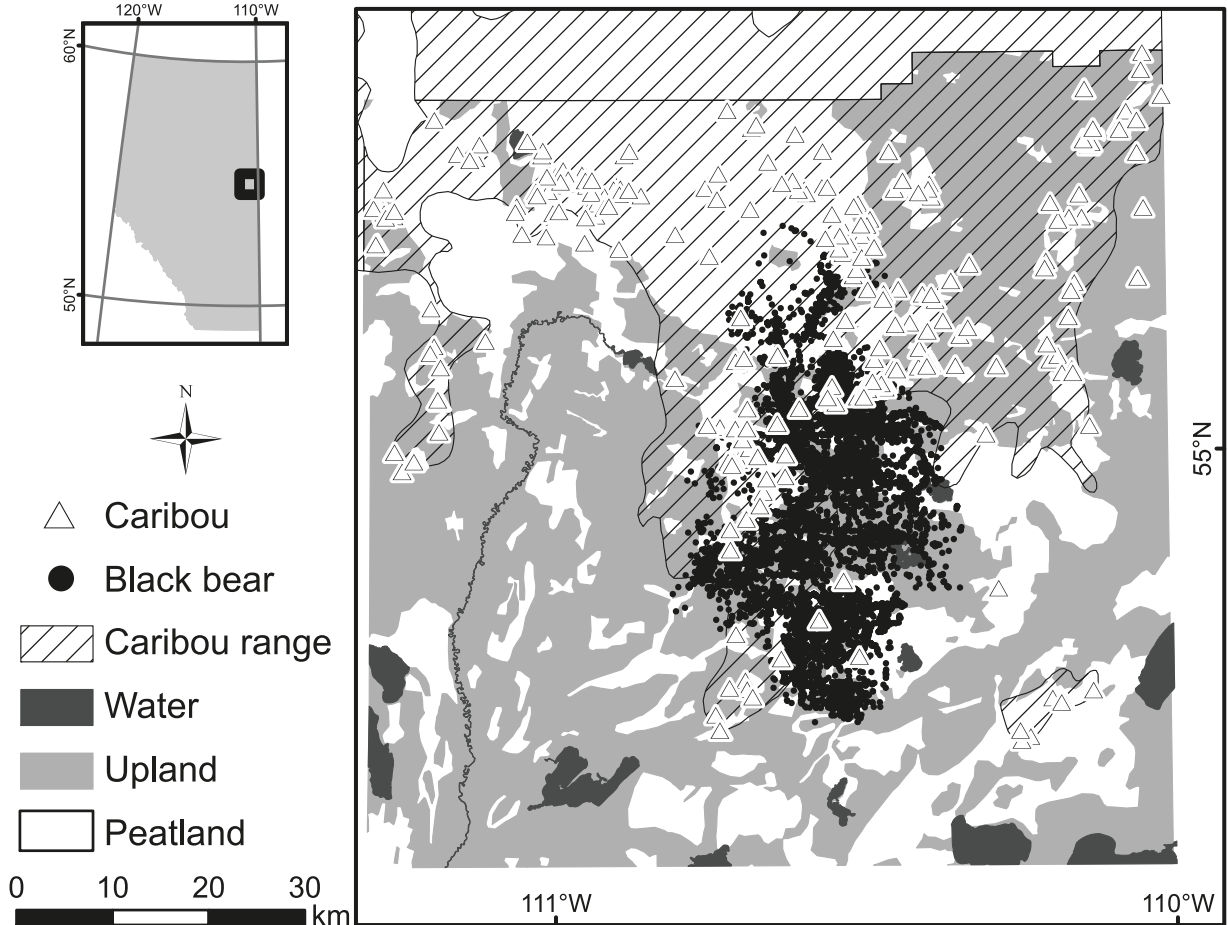
Fig. 1. The study area in the Cold Lake Air Weapons Range in northeastern Alberta, Canada. The town of Cold Lake is located directly to the south of the range (54°24'N, 110°12'W). Within this area, we radio-collared 15 black bears ( Ursus americanus ) and 37 adult female woodland caribou ( Rangifer tarandus caribou ) between 2001–2003 and 2000–2004, respectively.
